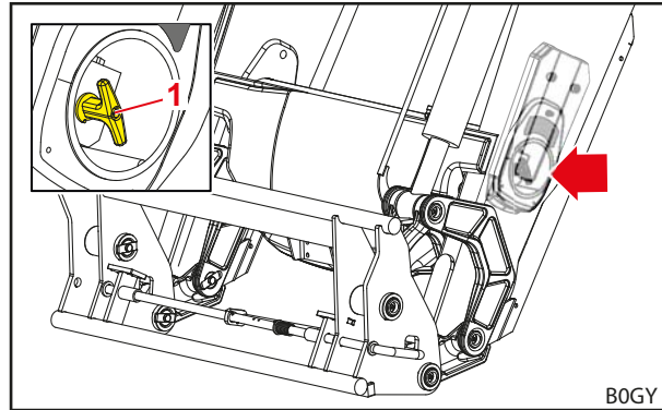
Mynd 38 Handstýrt Comfort-Drive
