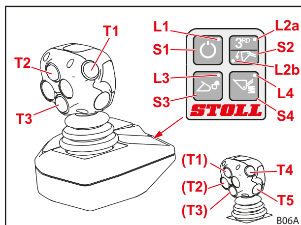
Att. 70 STOLL Pro Control
