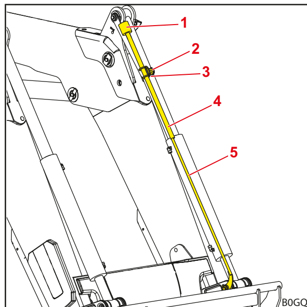
Att. 34 Return-To-Level sensors uz indikatora
