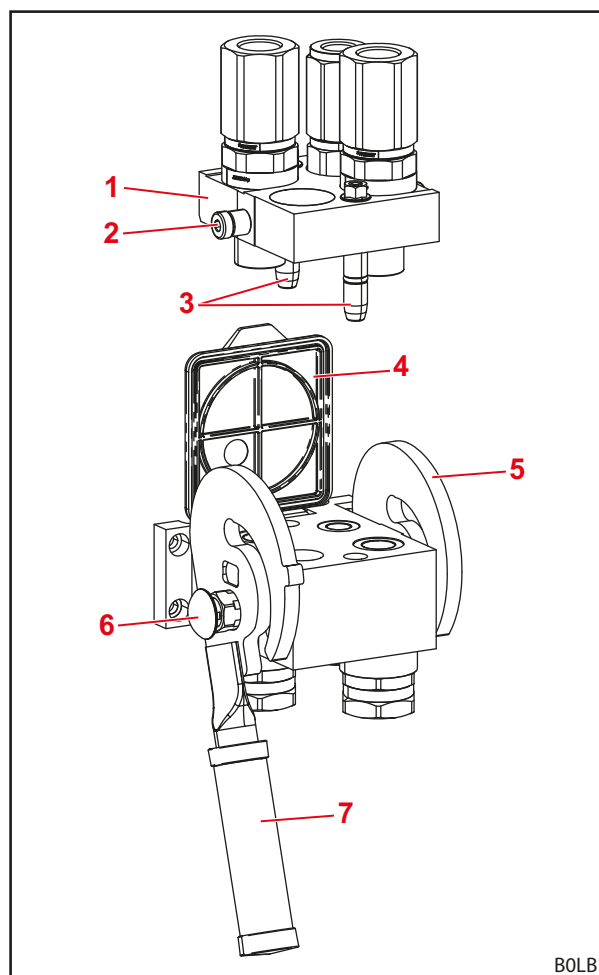
Rys. 73 Hydro-Fix
