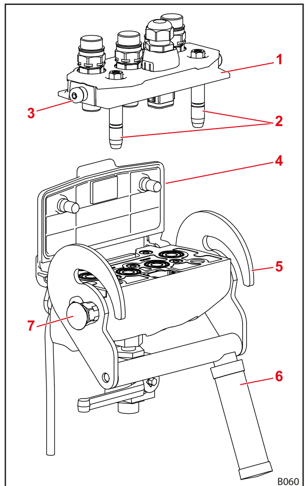
Rys. 77 Hydro-Fix
