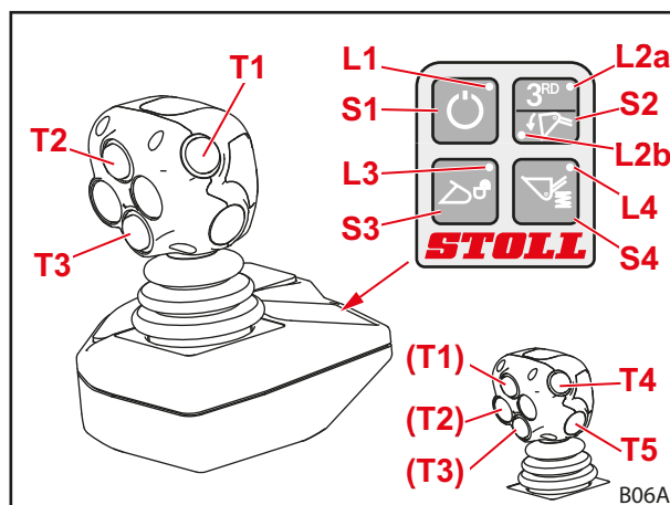
Rys. 51 STOLL Pro Control
