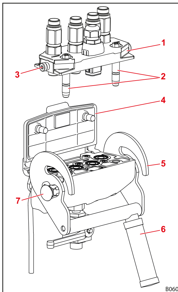
Fig. 74 Hydro-Fix (exemplu: Hydro-Fix 4)
