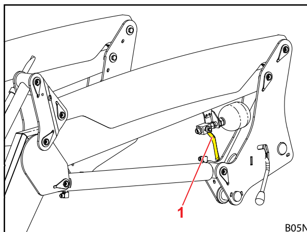
Sl. 40 Mehansko voden sistem Comfort Drive
