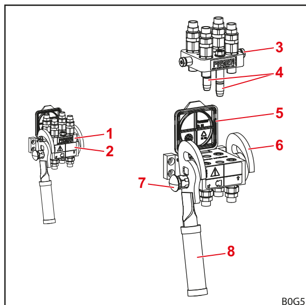
Obr. 17 Spojka Hydro-Fix
